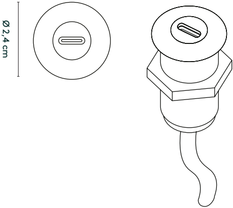
Integrated USB-C Port (Power & Data)
