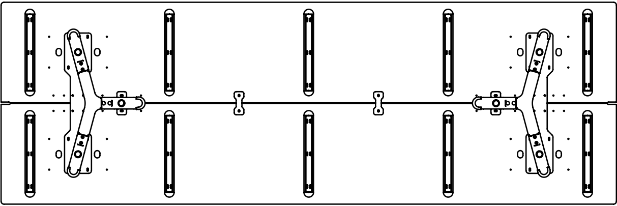
bottom view
